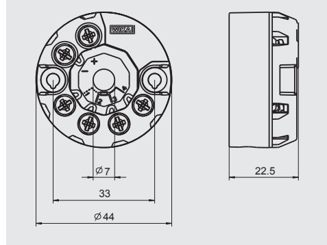
Head mounting version, model T15.H
