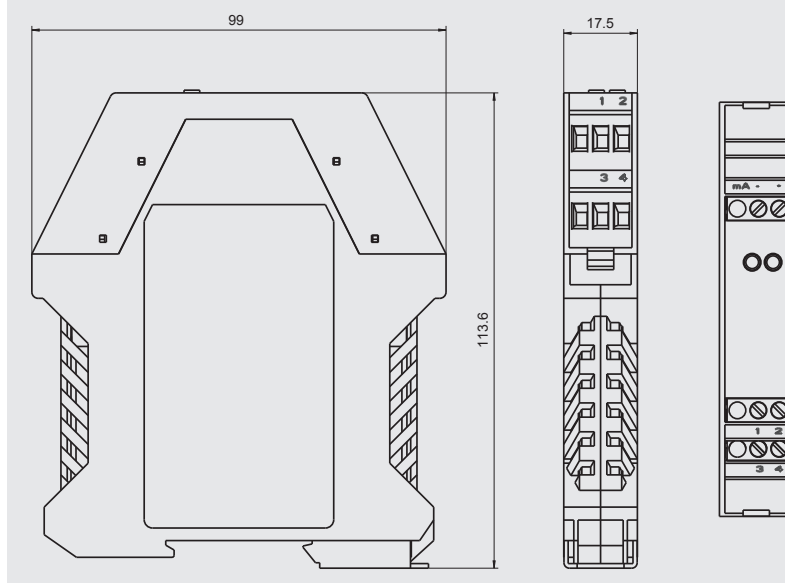
Rail mounting version, model T15.R
